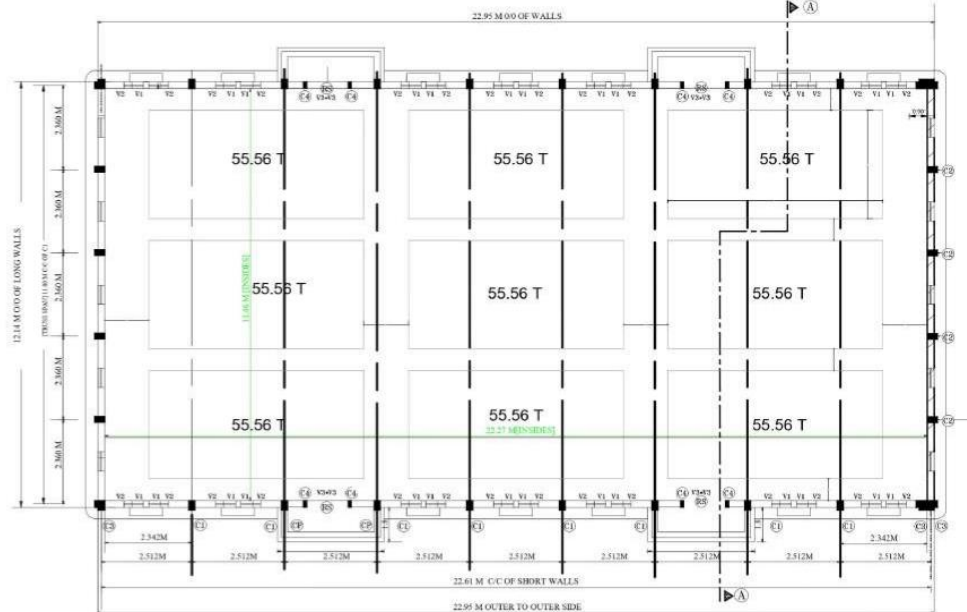
PLAN FOR 500 MT. WAREHOUSE UNIT NO. I, II
